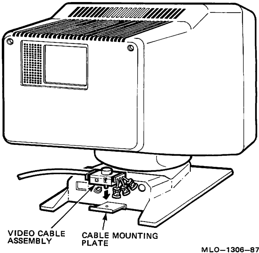
Figure 4: Mounting Video Cable Assembly on VR150 Monitor, Color Cable
